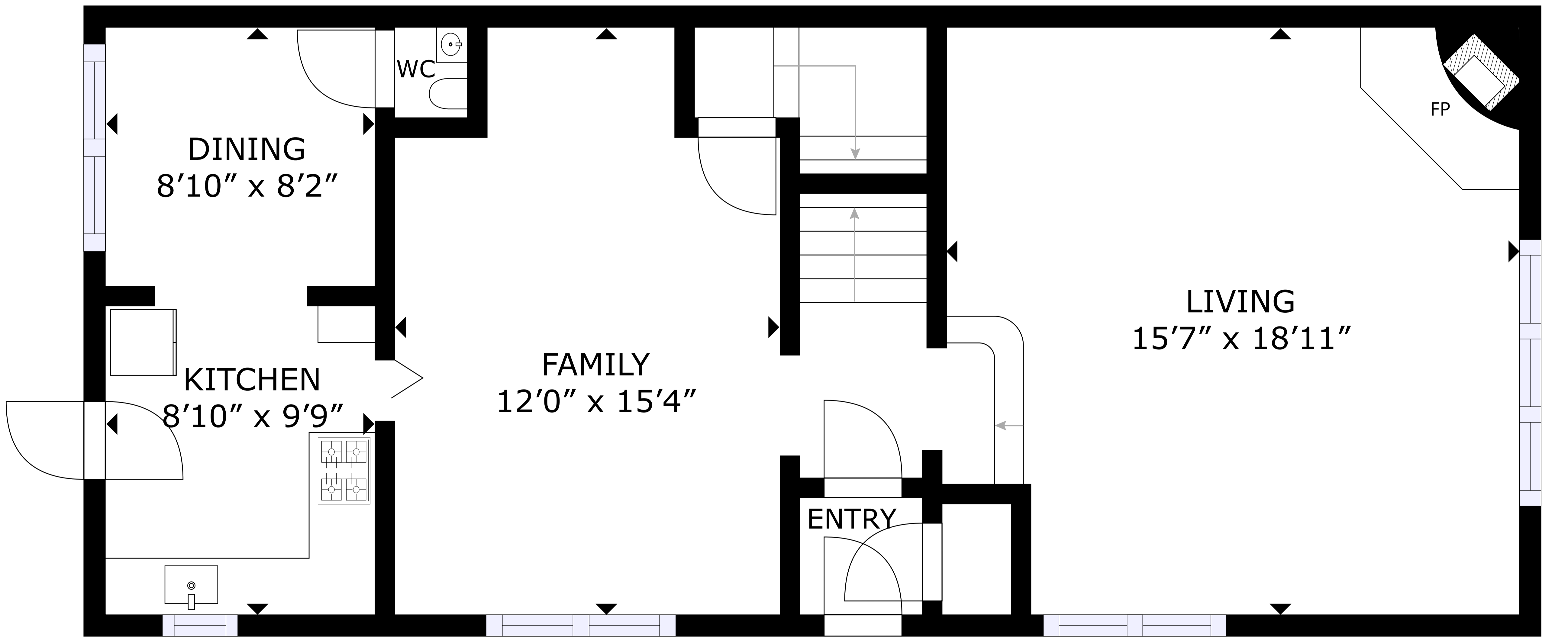
1ST FLOOR
